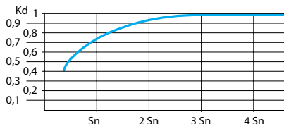
Typical curve for a steel object used with a cylindrical sensor
